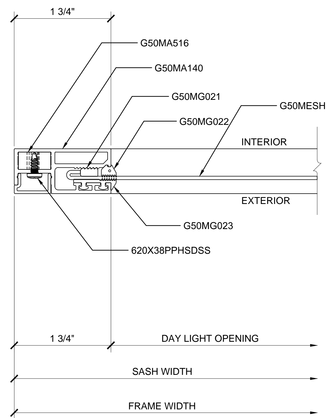
① SECTION DETAIL AT JAMB
