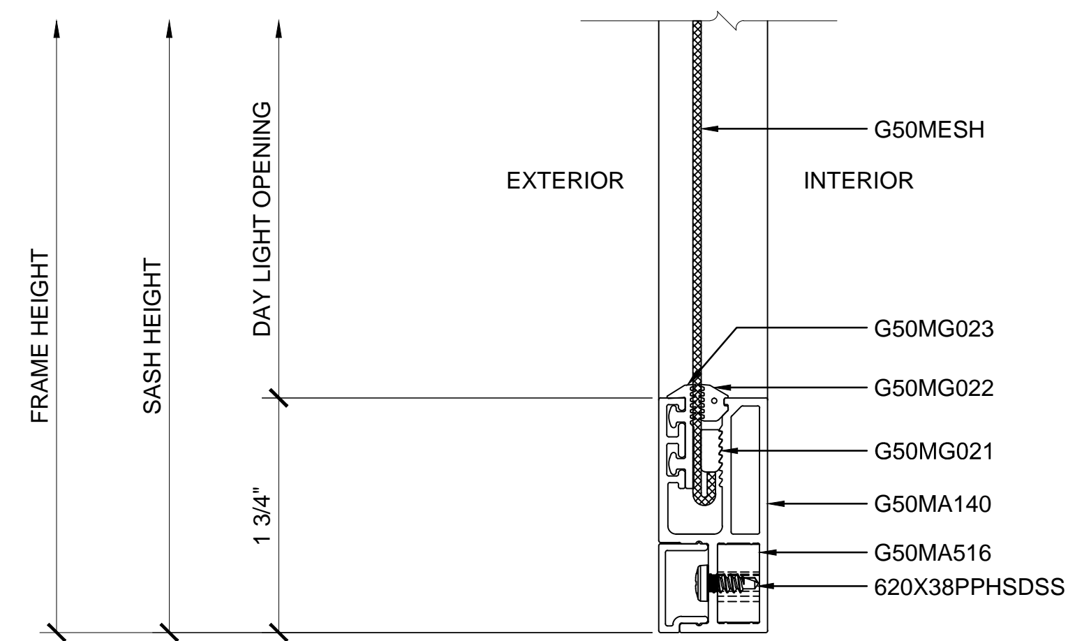
2 SECTION DETAIL AT SILL
