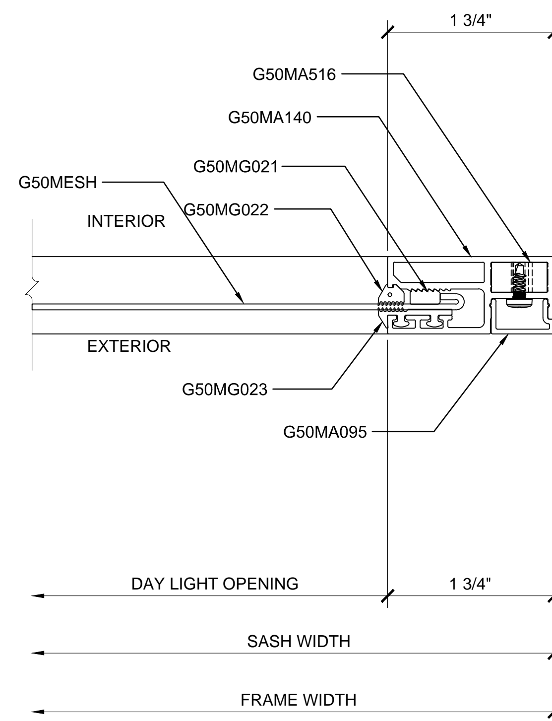
② SECTION DETAIL AT JAMB
